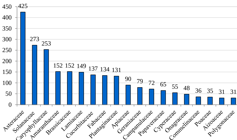
Fig. 4. Species numbers of the most diverse families in the JHDC
